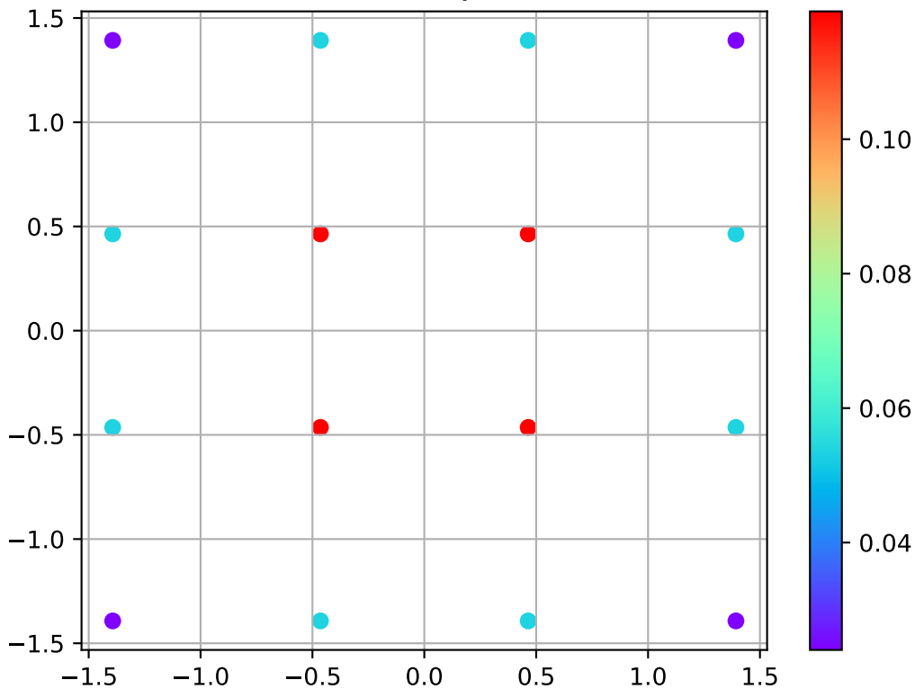
16-PCS-QAM
