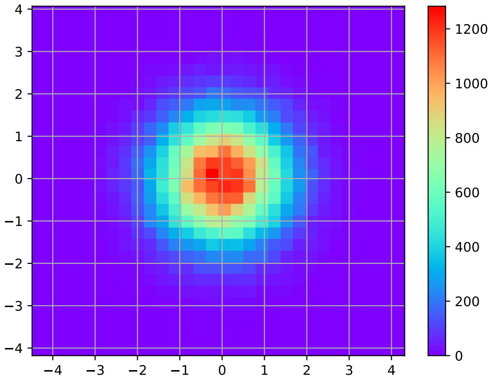
Gaussian
