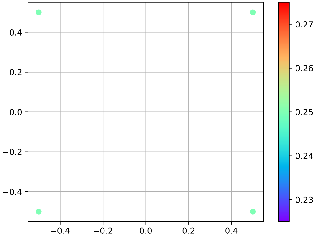
4-Binomial-QAM
